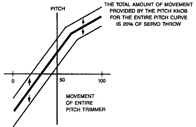
OVERALL PITCH TRIM CONTROL OPERATION
