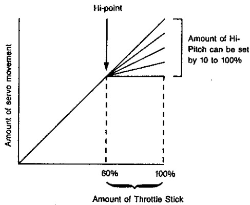
Movement of Pitch Curve
